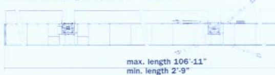
Basic mast climbing work platform Extension
