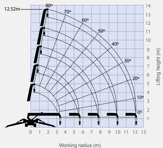
The Working Range Chart does not take into account boom deflection under load.
