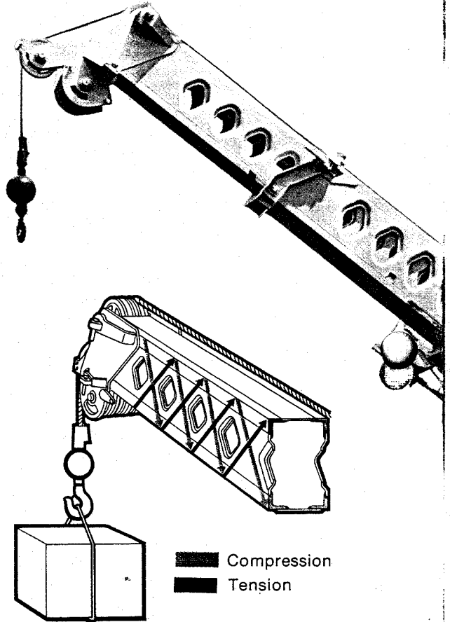
FMC's exclusive boom design (patented)
