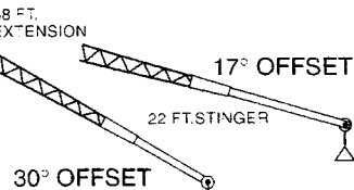
30° OFFSET
