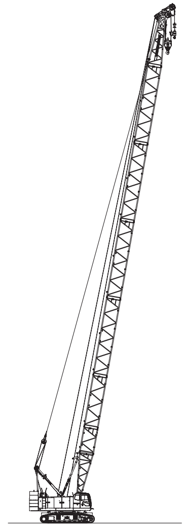
Crane Specification (Boom Longest Length with Aux. Sheave)
