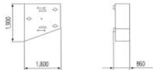
Counterweight
