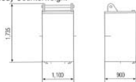
Carbody Counterweight
