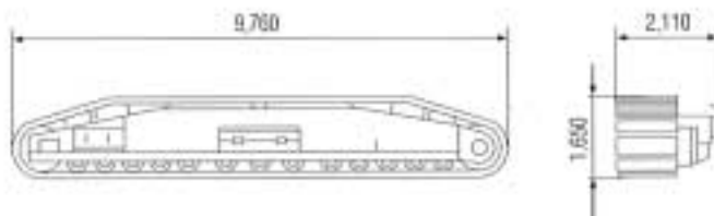
Crawlers
